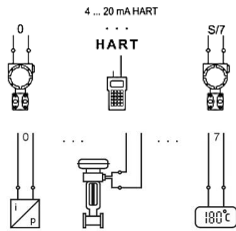
Approved i/p converters, positioners, indicators
