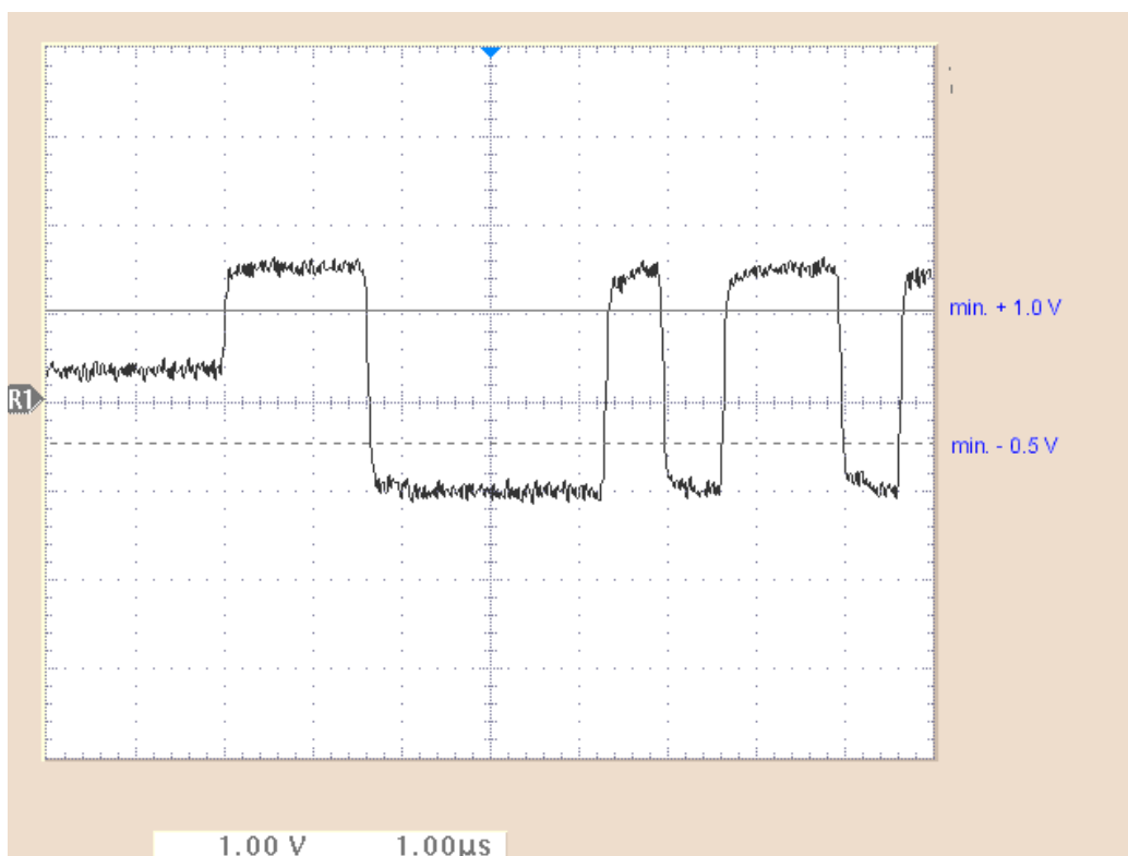
Fig 11 Minimum transmission levels on the RS 485 Ex i bus in accordance with R. STAHL Specification. The level should be above + 1 V and below – 0.5 V. The quiescent level is approx. 0.2 to 0.3 V in the case of a correctly terminated bus.
