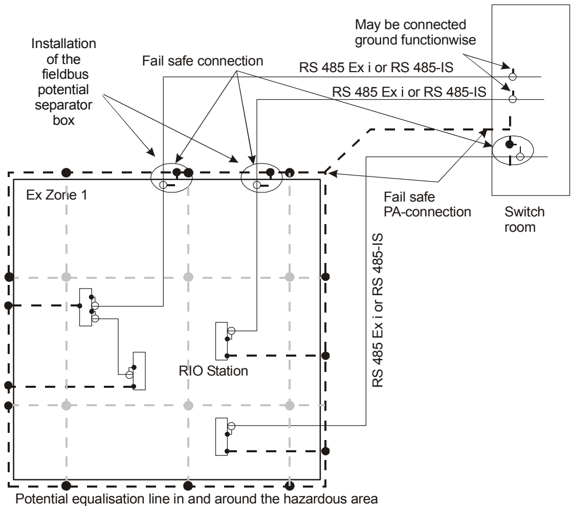
Fig 7 Earthing of a conductive shield
