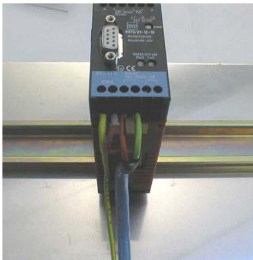
Fig 6 Connection of the external resistor
