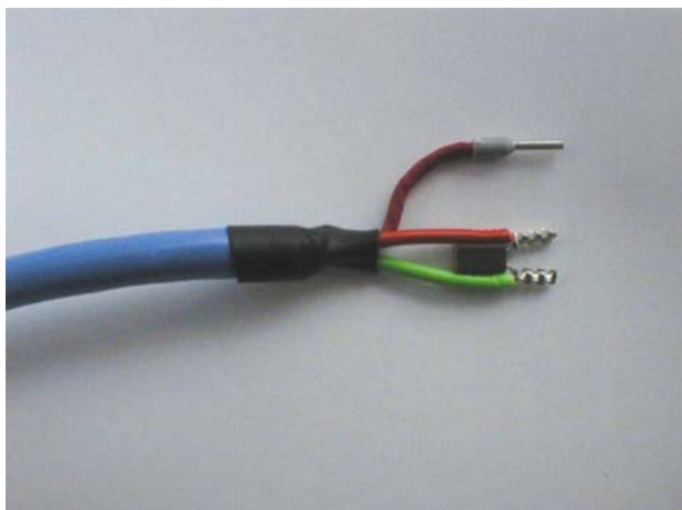
Fig 5 external 470 Ohm resistor
