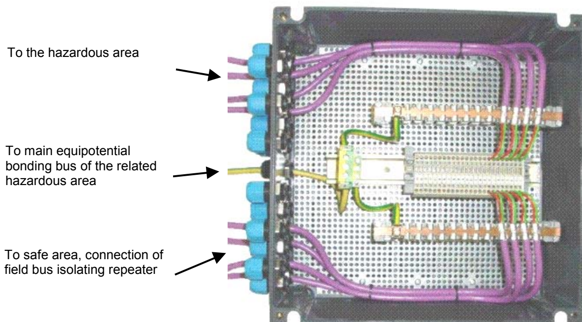
Fig 8 Example of a fieldbus potential isolating box
