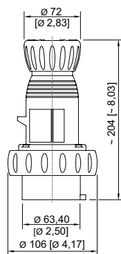
5-pole plug
