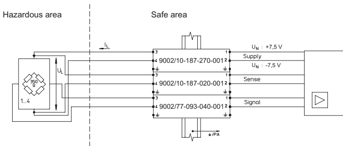
Application: Load cell (DMS) 350 \Omega or 700 \Omega 6-wire \pm 7.5 V (15 V) field circuit unearthed
