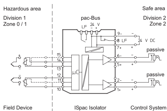
Connection diagram 9182/20-51-11
