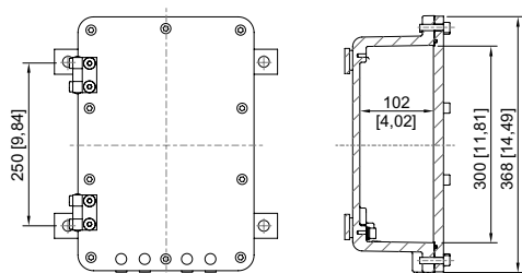
Enclosure size 2
