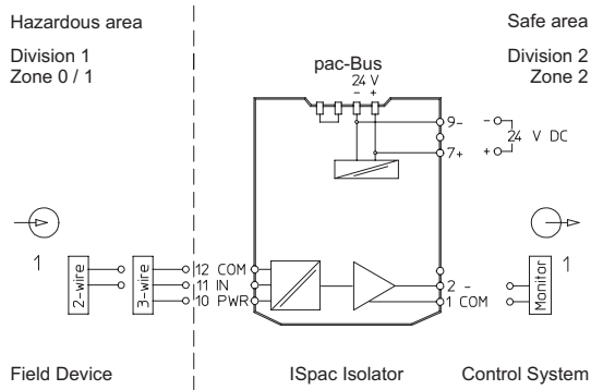
Connection diagram 9147/10-99-10
