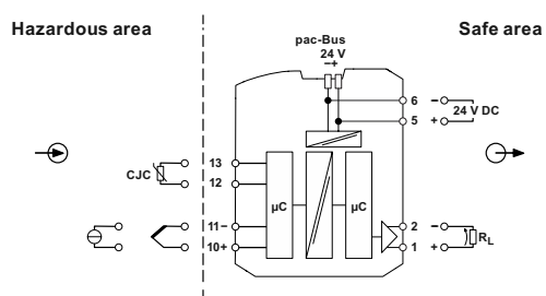
9282/12-51-16 connection diagram
