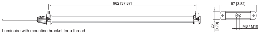
Luminaire with mounting bracket for a thread
