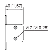
Mounting bracket for a thread
