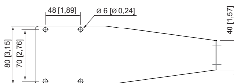
Mounting bracket for a thread
