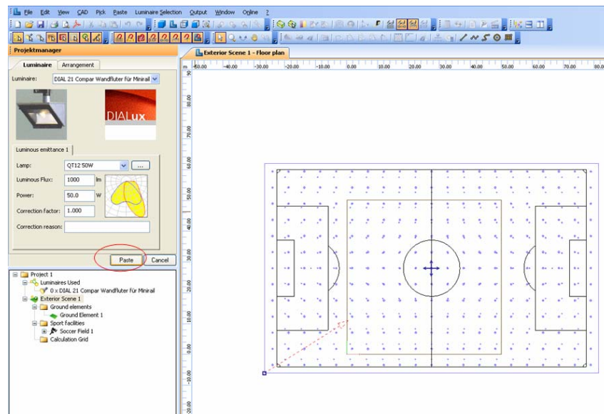
Fig. 163 Inserting floodlight illumination in a sports complex
