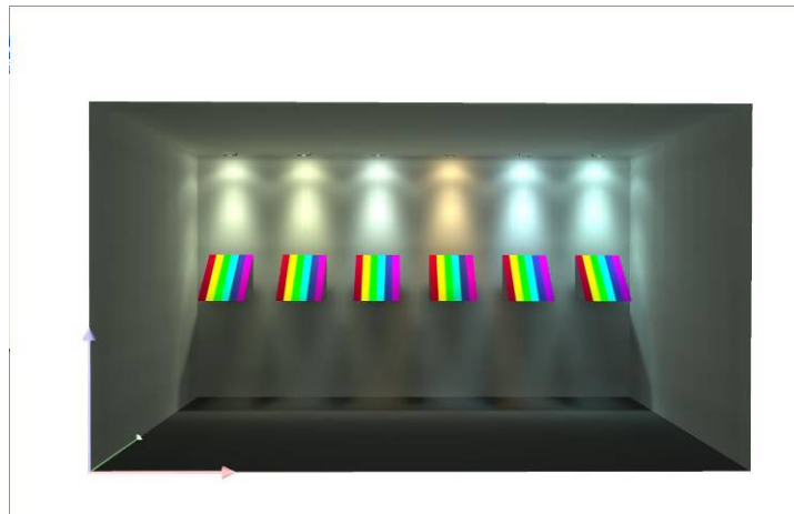
Fig. 205 All the spots are using the same colour filter, but have different light sources. From the left: Incandescent, Fluorescent 830, D65, high pressure sodium, metal halide ceramic and metal halide quartz
