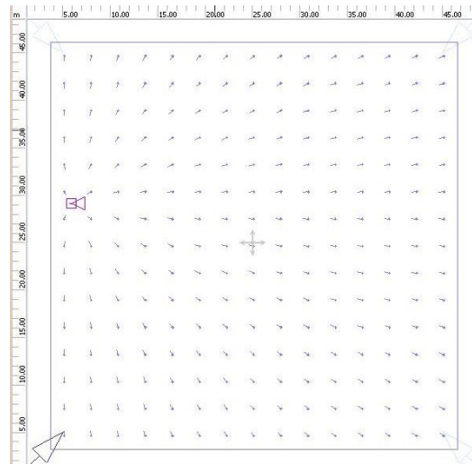
Fig. 337 CAD output of camera-oriented luminous intensity
